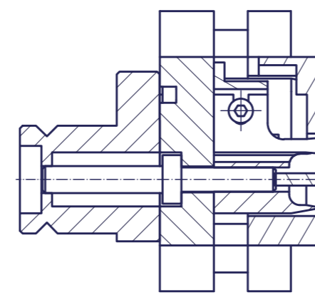
B-B (1:1)
