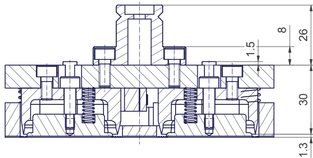
B-B (1:1)
