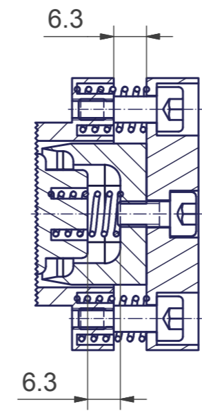
B-B (1:1)
