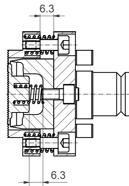
B-B (1:1)
